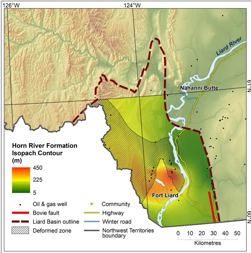
Figure 3: Gross thickness of the Horn River Formation in the Liard Basin varies from 5 m to 450 m between 60°N and 61°N. The Horn River Formation overlies Nahanni Formation carbonate rocks that form the reservoir for conventional natural gas in the Pointed Mountain and Liard fields (see Figure 11). The Horn River Formation is thickest near Pointed Mountain and thins abruptly east of the Bovie fault.
