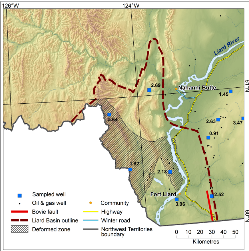
Figure 5: Organic richness of the Horn River Formation in average weight percent total organic carbon (TOC) from sampled wells. Data are limited and there are no apparent TOC trends within the Liard Basin. TOC data were obtained from wells sampled by the NTGS and the Geological Survey of Canada (GSC; Potter et al., 2000; Feinstein et al., 1988).
